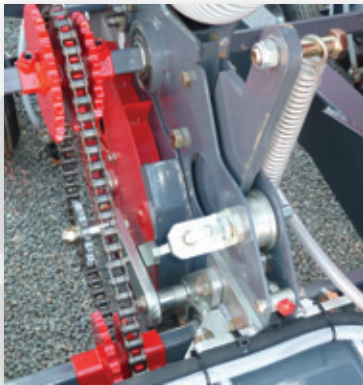
Central gear box for density choice
